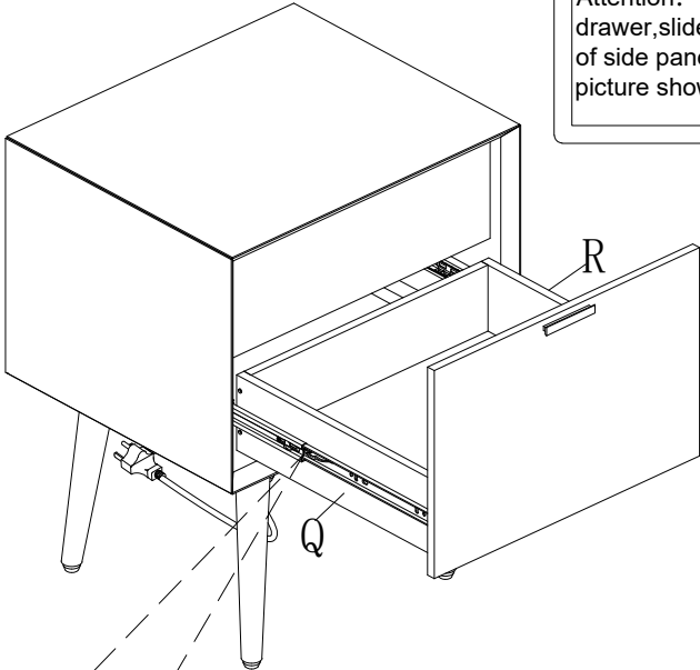
Schematic diagram of slide rail disassembly
