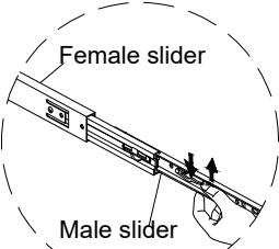
Schematic diagram of slide rail disassembly
